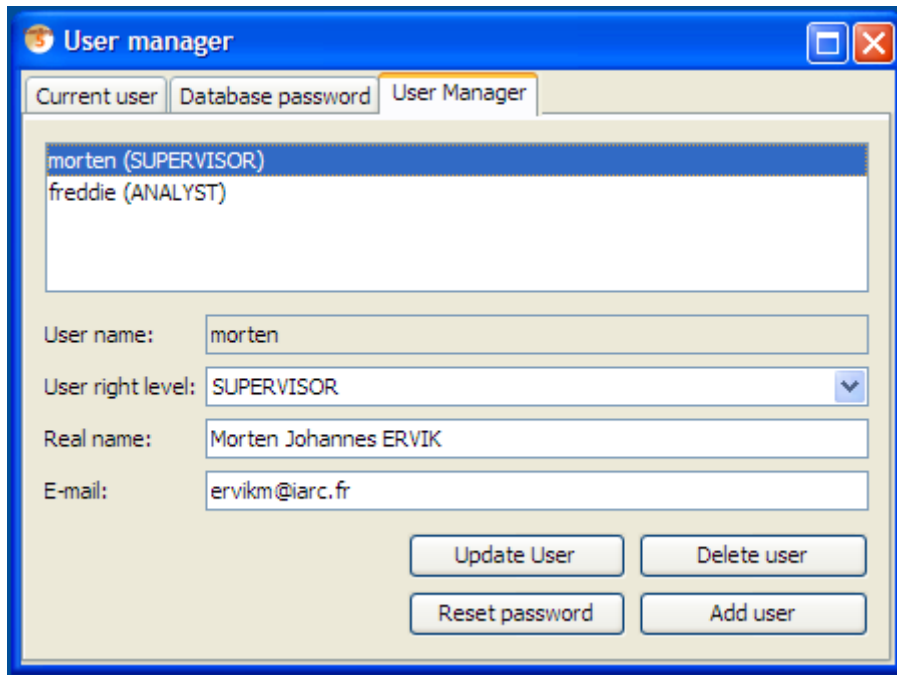
Figure 7.3.: User manager
